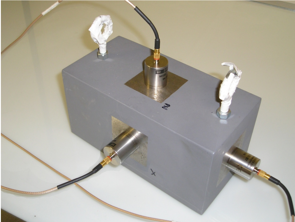
Figure 2: 35 lb. steel block with three mounted accelerometers.
