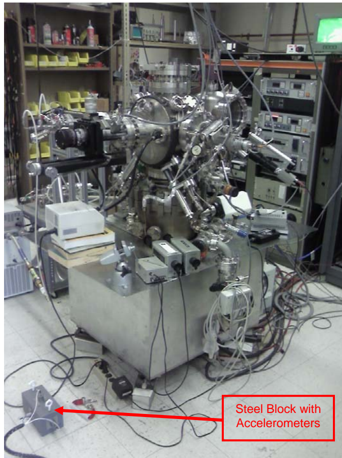
Figure 4: Vibration measurement set up for scanning tunneling microscope.
