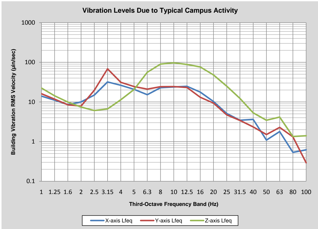
Figure 5: Tri-axial time averaged vibration levels.
